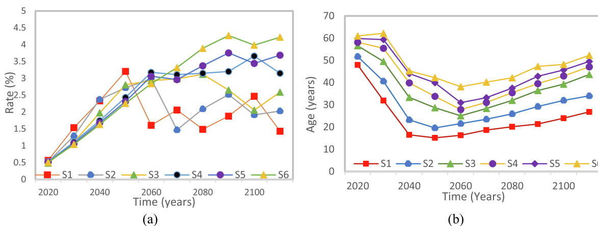
Fig. 4. The rate (%) of broadleaved species (a) and the average stand age (b) over 100 years.
