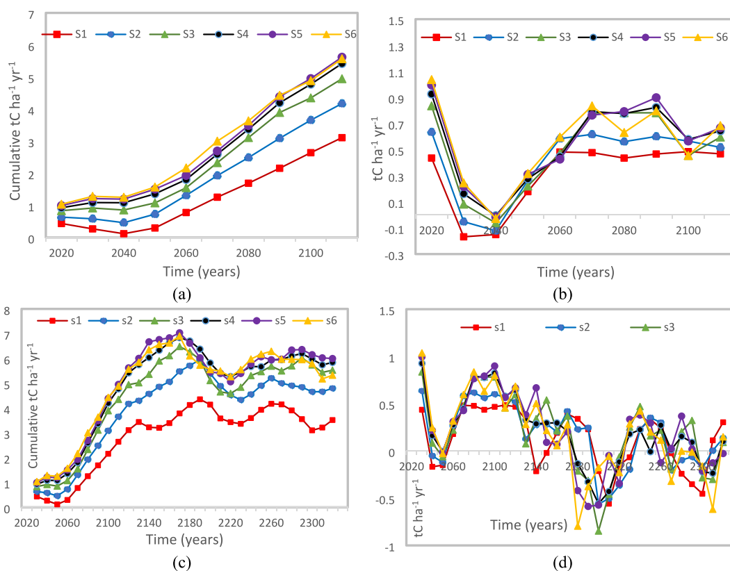
Fig. 7. Cumulative stored carbon in tons ha -1 year -1 (a) and carbon balance in tons ha -1 year -1 (b) over 100 years. Similarly, the cumulative stored carbon in tons ha -1 year -1 (c) and carbon balance in tons ha -1 year -1 (d) over 300 years.
