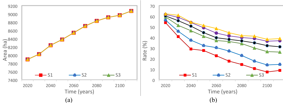
Fig. 5. The change of forest land with afforestation (a) and the rate (%) of understory (b) over 100 years.
