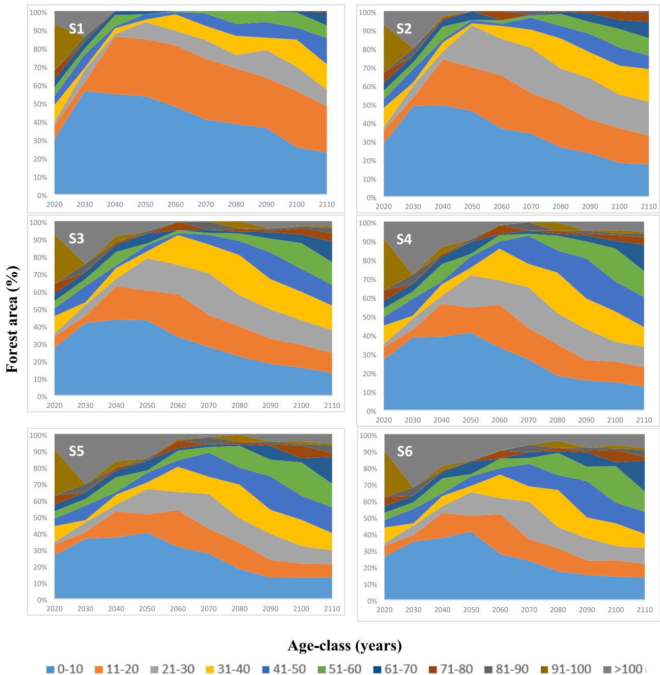
Fig. 1. The development of forest area (ha) by age-class over 100 years of simulation for six management scenarios.
